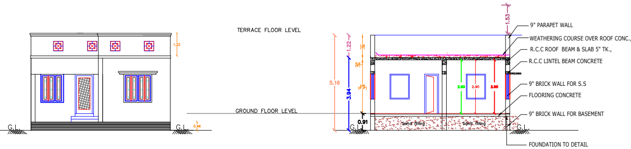
FRONT ELEVATION
