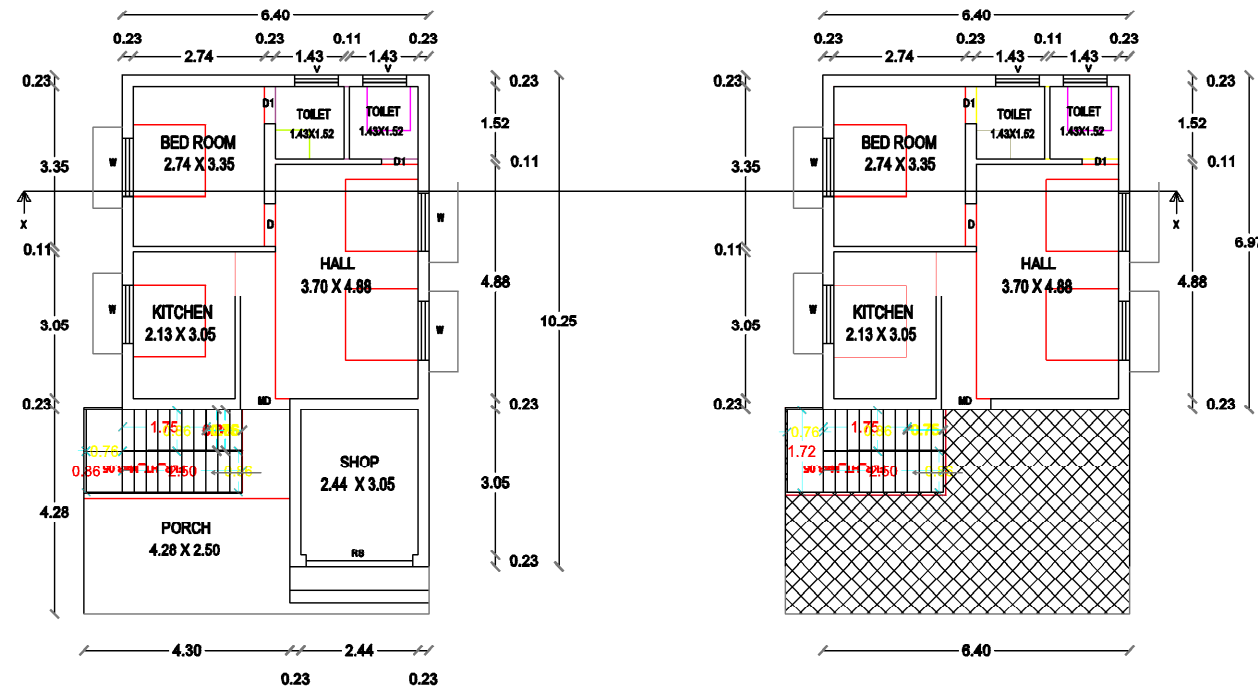
EXG - GROUND FLOOR PLAN
