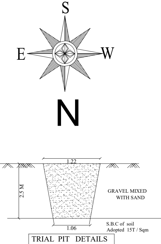
TRIAL PIT DETAILS
