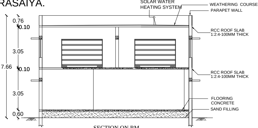
SECTION ON RM
