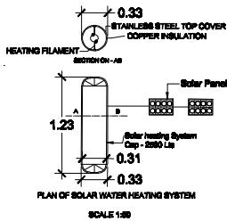
SCALE 1:80
