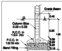
COLUMN DETAILS NOT TO SCALE
