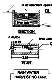
RAIN WATER HARVESTING TANK
