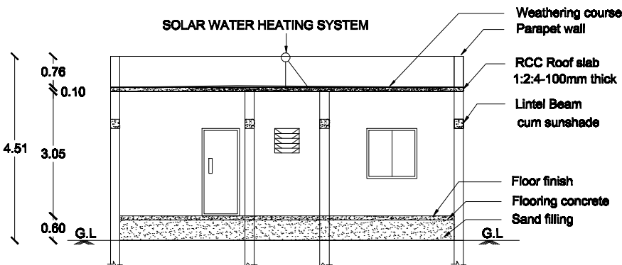
SECTION ON MK
