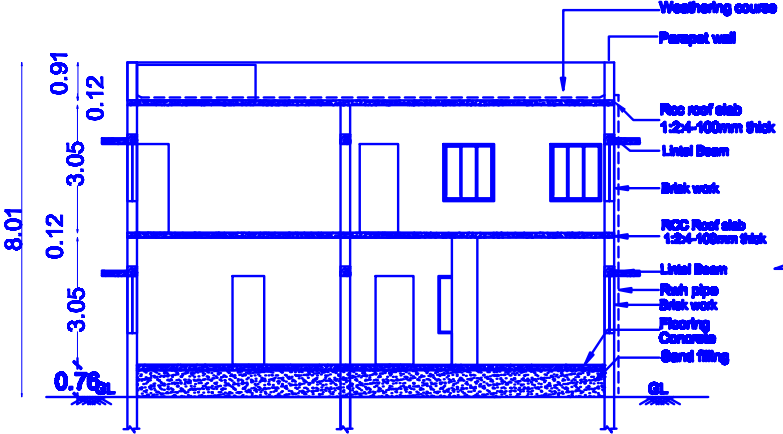
SECTION -XY
