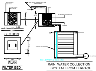
RAIN WATER COLLECTION SYSTEM FROM TERRACE
