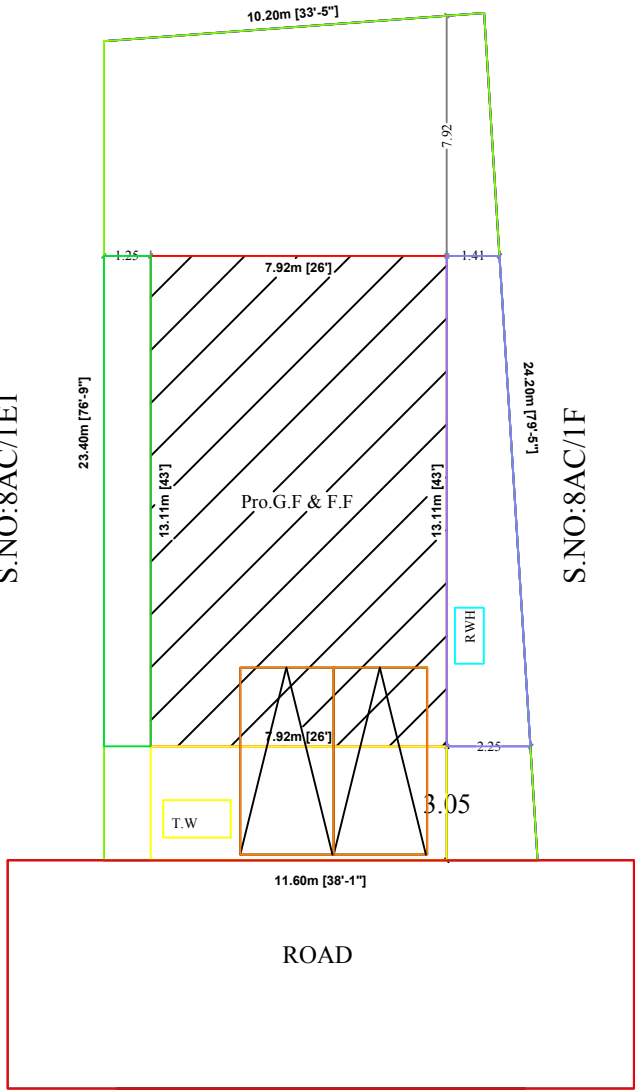
SITE PLAN
