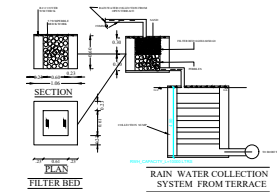
RAIN WATER HARVESTING 1. PERCOLATION PIT
