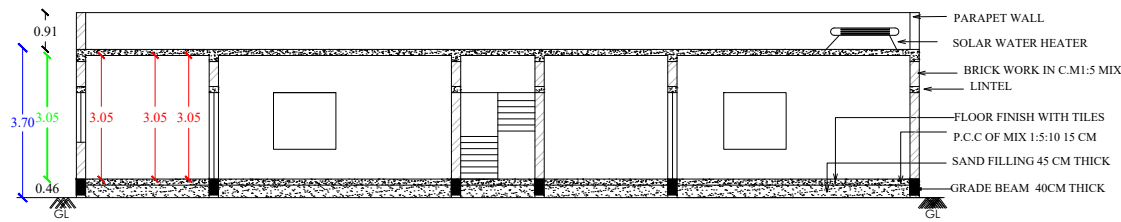
SECTION- AA1
