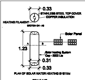
PLAN OF SOLAR WATER HEATING SYSTEM SCALE 1:50
