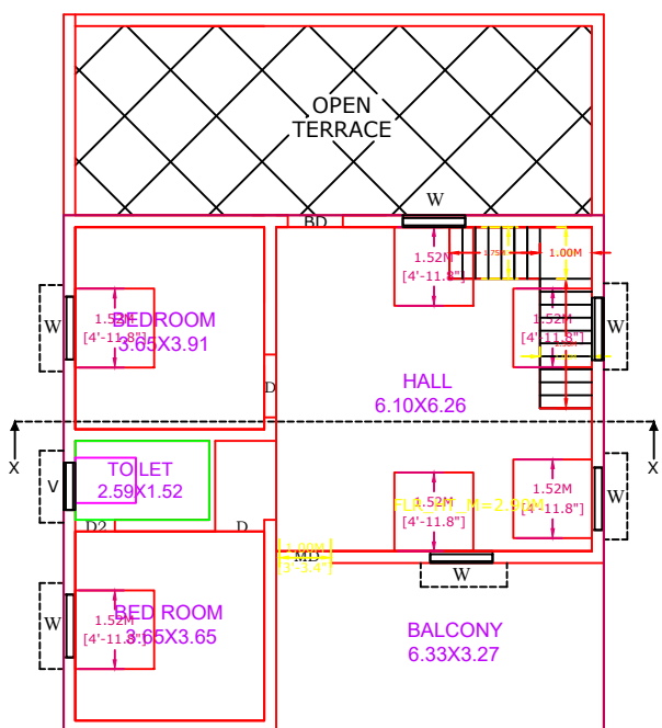
EXIS.FIRST FLOOR PLAN
