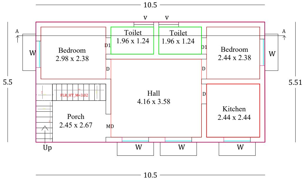
PRO.GROUND FLOOR PLAN
