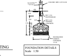
FOUNDATION DETAILS Scale 1:50
