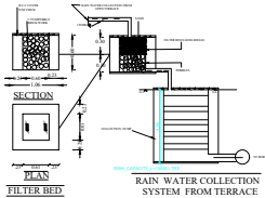
RAIN WATER HARVESTING I.PERCOLATION PIT
