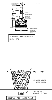
FOUNDATION DETAILS Scale 1:50
