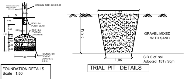
SECTION-AA1
