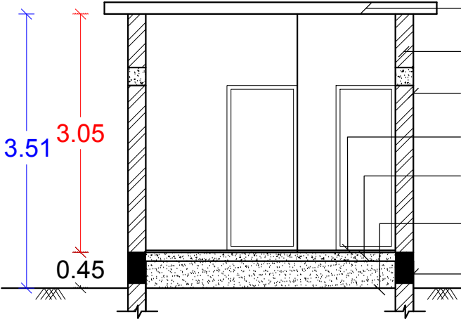
SECTION-AA1
