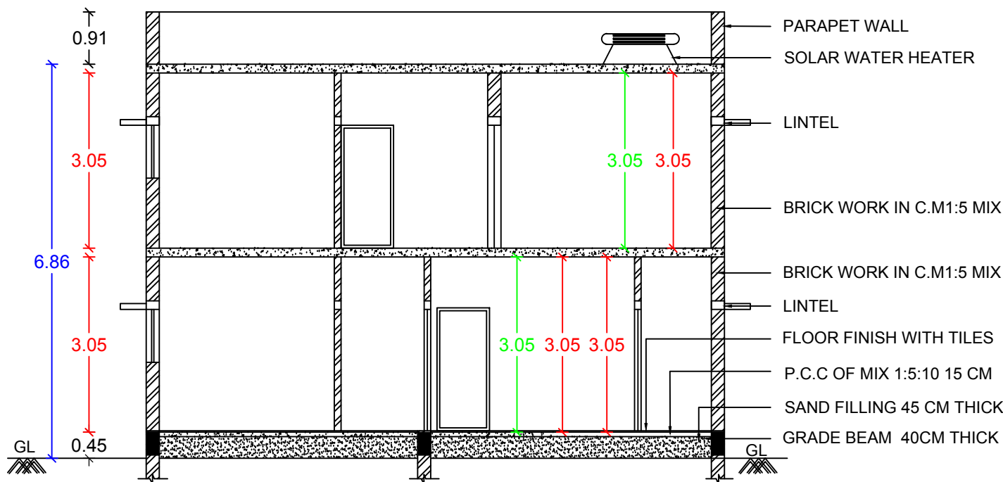
SECTION- AA1
