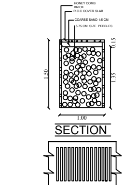
RAIN WATER HARVESTING PERCOLATION BED
