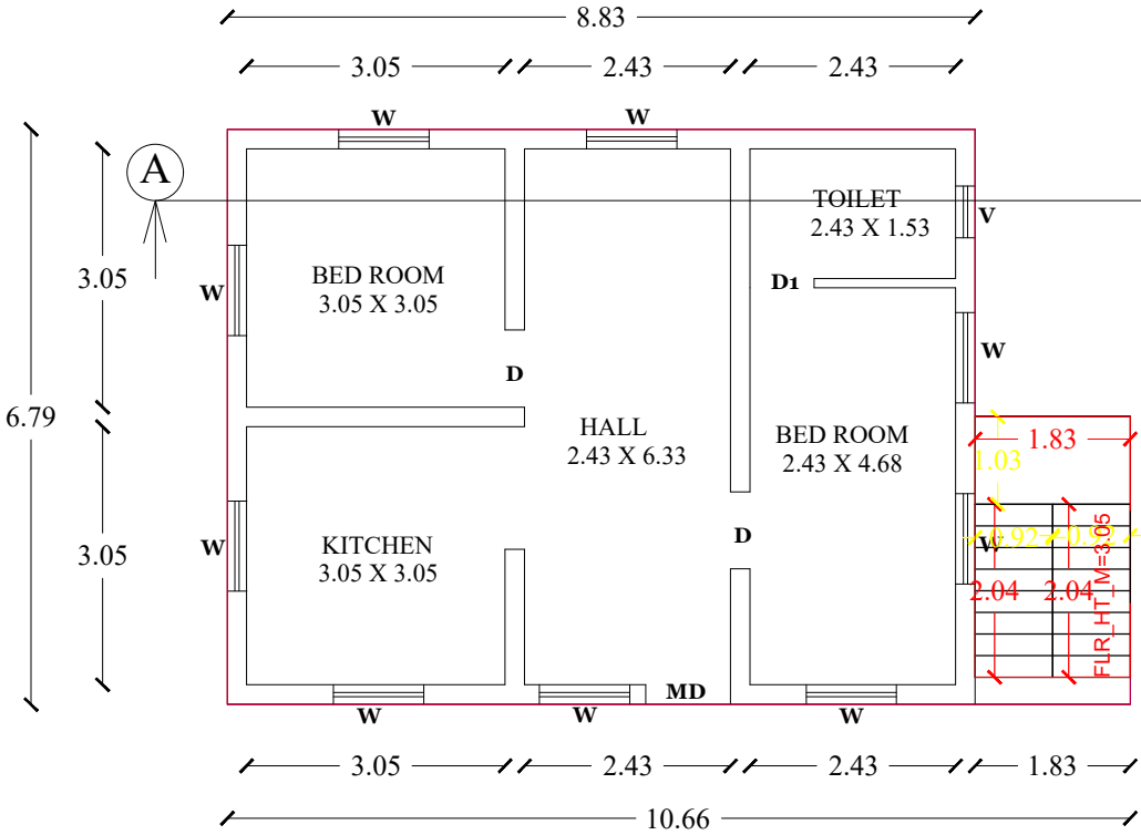
EXI. GROUND FLOOR PLAN
