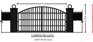
COMPOUND GATE (NOT TO SCALE)
