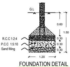
FOUNDATION DETAIL
