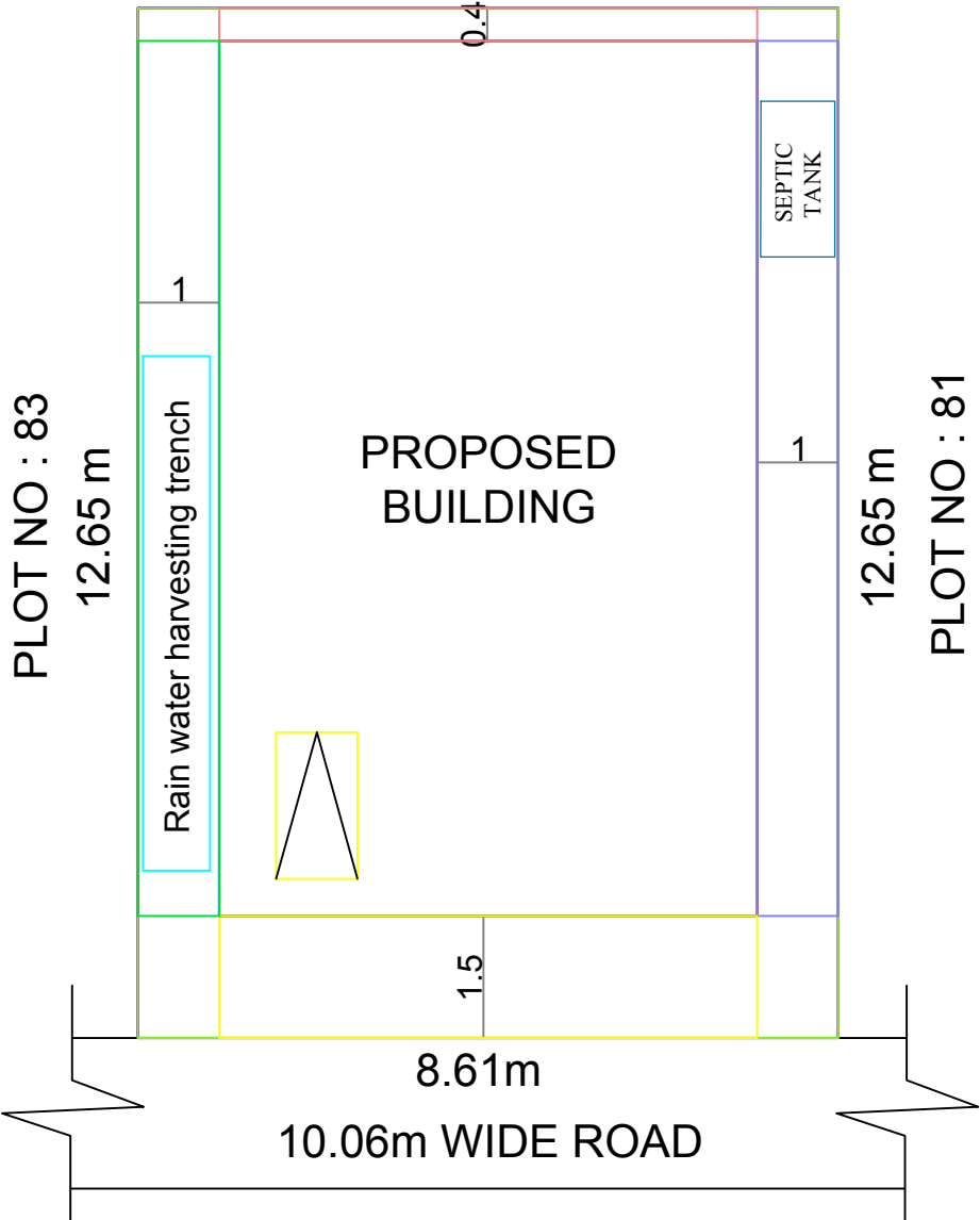
SITE PLAN
