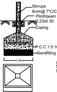
Foundation Details
