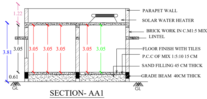
SECTION- AA1
