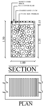
RAIN WATER HARVESTING PERCOLATION BED
