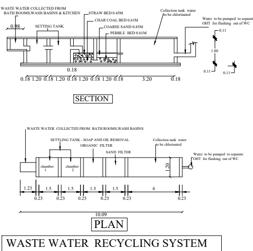
WASTE WATER RECYCLING SYSTEM
