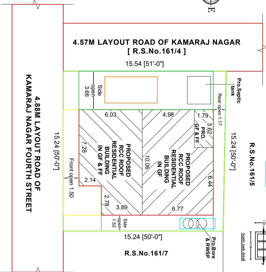
SITE PLAN
