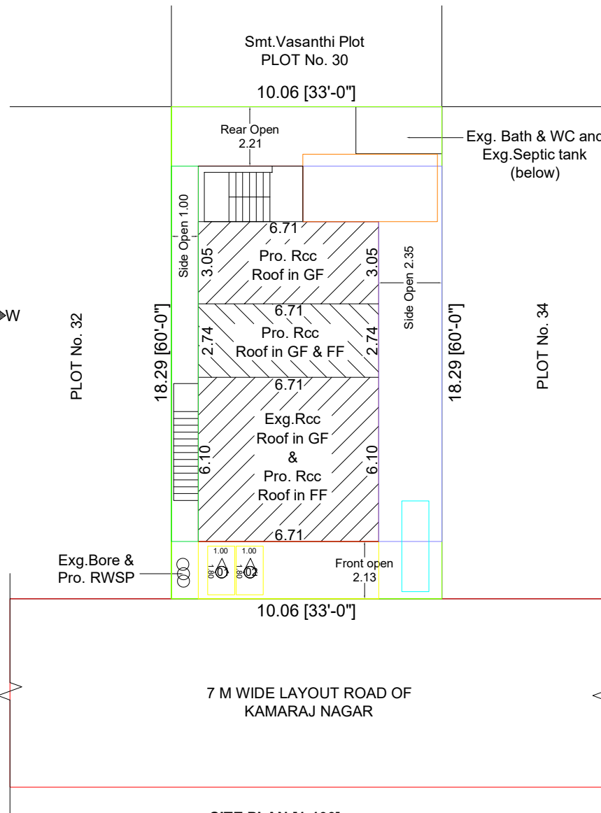
SITE PLAN [1:100]
