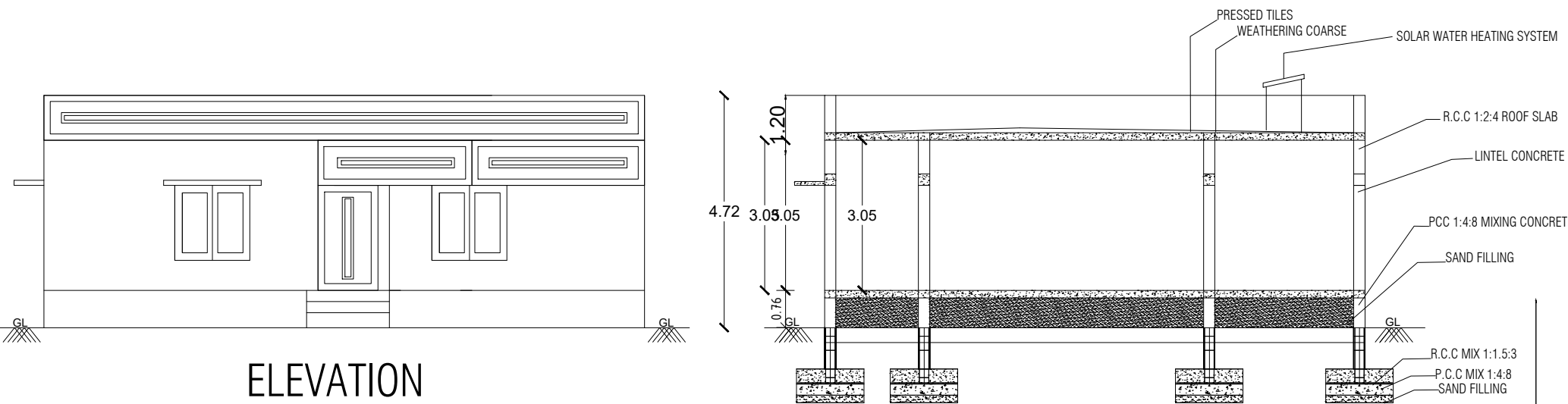
SECTION NO -"AA"
