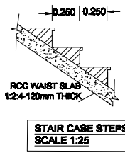
STAIR CASE STEPS SCALE 1:25
