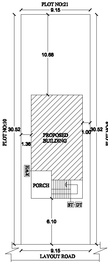
SITE PLAN SCALE 1:200
