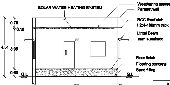
SECTION ON MK
