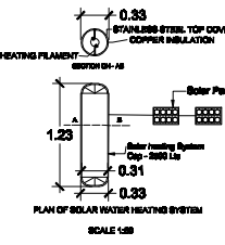
PLAN OF SOLAR WATER HEATING SYSTEM SCALE 1:50
