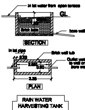
RAIN WATER HARVESTING TANK
