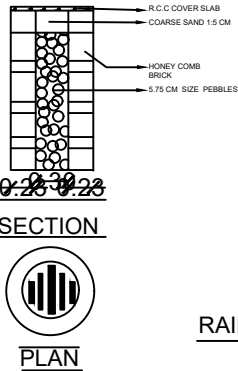
1. PERCOLATION PIT
