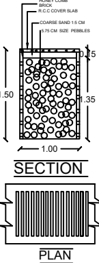
RAIN WATER HARVESTING PERCOLATION BED
