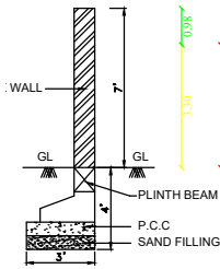
FOUNDATION WALL DETAIL
