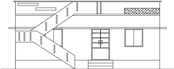
FRONT ELEVATION
