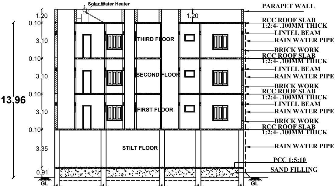
SECTION - A B
