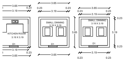
PROPOSED COMMERCIAL G.FLOOR RESTAURENT
