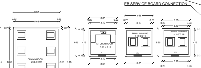
PROPOSED COMMERCIAL G.FLOOR RESTAURENT
