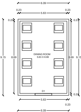
PROPOSED COMMERCIAL G.FLOOR SHEDWORK GROUND FLOOR PLAN
