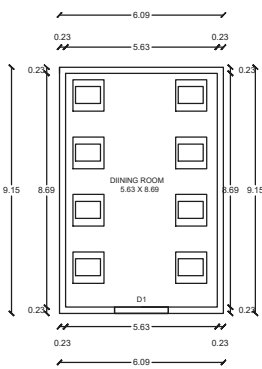
PROPOSED COMMERCIAL G.FLOOR SHEDWORK GROUND FLOOR PLAN
