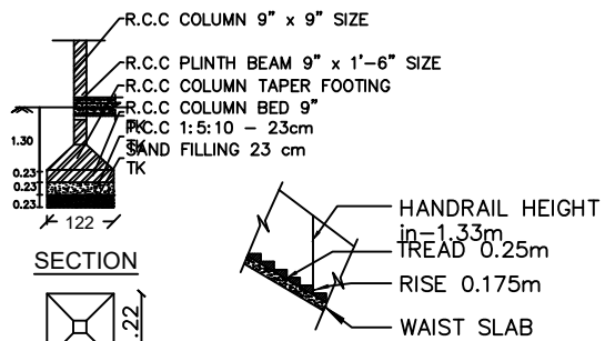
COLUMN DETAILS PLAN
