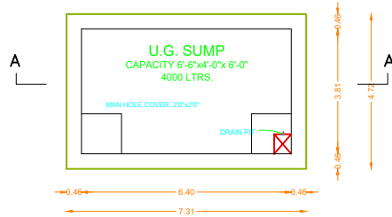
SUMP DETAIL
