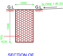
SECTION OF PEBBLE TRENCH SCALE : 1: = 100
