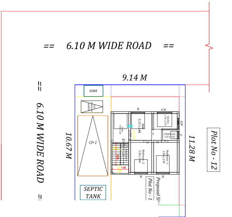
Compound Wall - Plan
