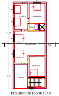
PRO. GROUND FLOOR PLAN
