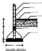
COLUMN DETAIL
