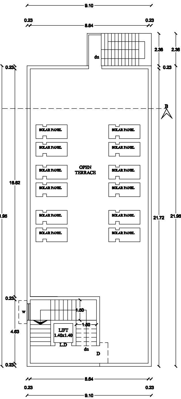
PRO-TERRACE FLOOR PLAN
