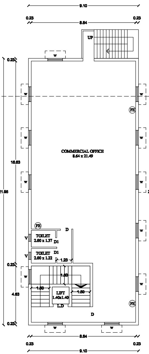
TYPICAL SECOND & THIRD FLOOR PLAN
