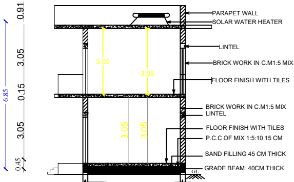
SECTION-AB
