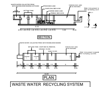
WASTE WATER RECYCLING SYSTEM
