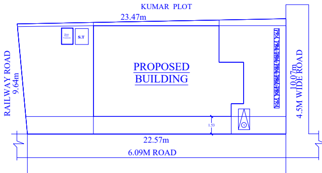
SITE PLAN SCALE 1:200
