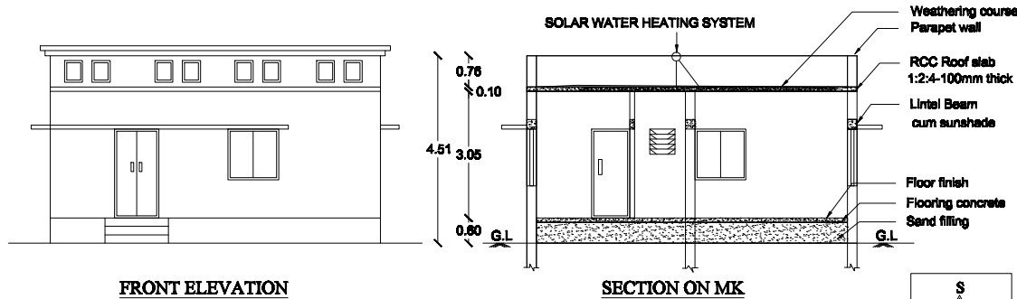
FRONT ELEVATION
