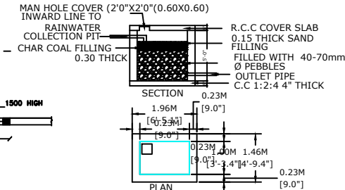
RWH_CAPACITY_L=5000LTRS
