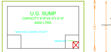
SUMP DETAIL
