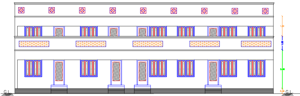
FRONT ELEVATION
