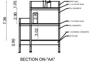
SECTION ON-AA'
