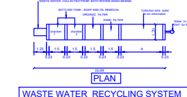
PLAN WASTE WATER RECYCLING SYSTEM
