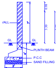
FOUNDATION WALL DETAIL
