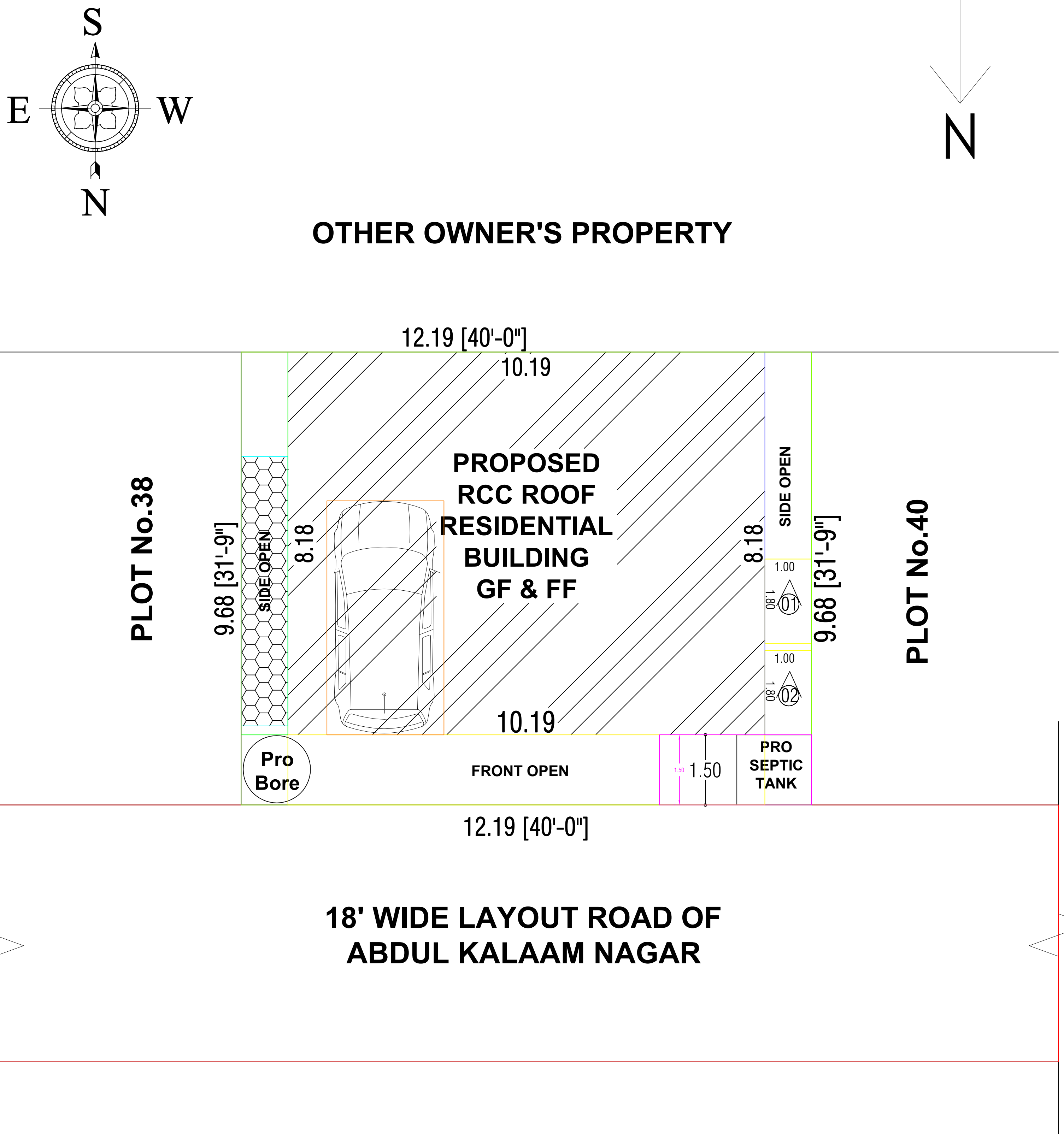
SITE PLAN [1:100]
