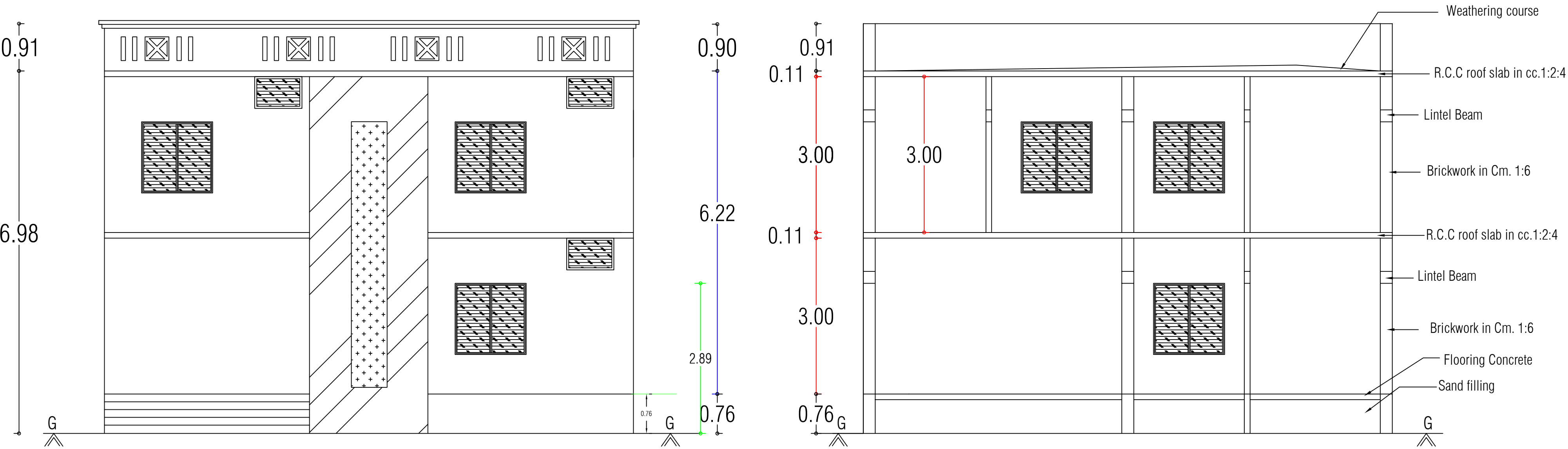
FRONT ELEVATION
