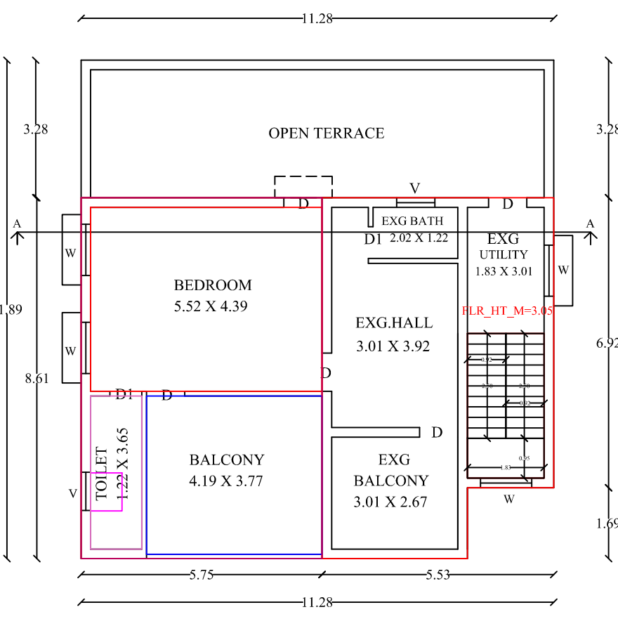
PROPOSED & EXISTING FIRST FLOOR PLAN
