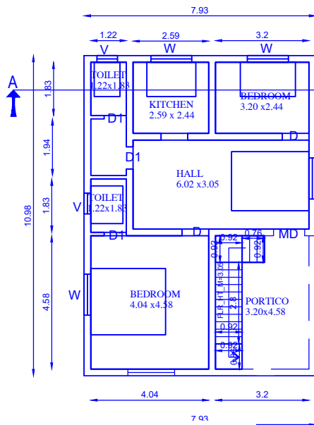
PLAN
