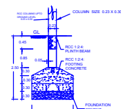
FOUNDATION DETAILS Scale 1:50
