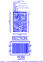
RAIN WATER HARVESTING PERCOLATION BED
