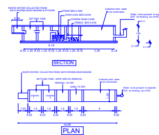
WASTE WATER RECYCLING SYSTEM
