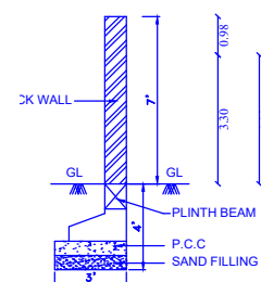
POUND WALL DETAIL
