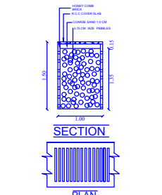
RAIN WATER HARVESTING PERCOLATION BED
